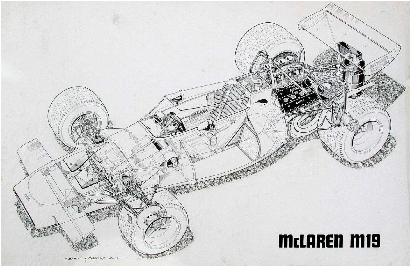
McLaren M19 cutaway for the Autocar
