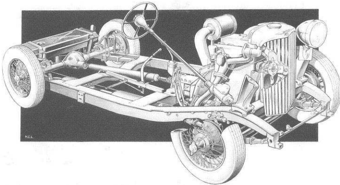
Jaguar 1.5 litre chassis for the motor magazine September 1945 Image courtesy of Ian Cooling
