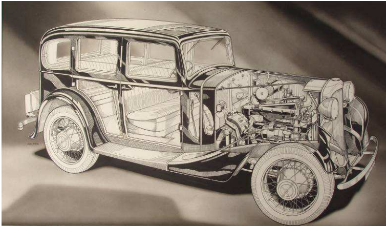
1933 Hillman Saloon
