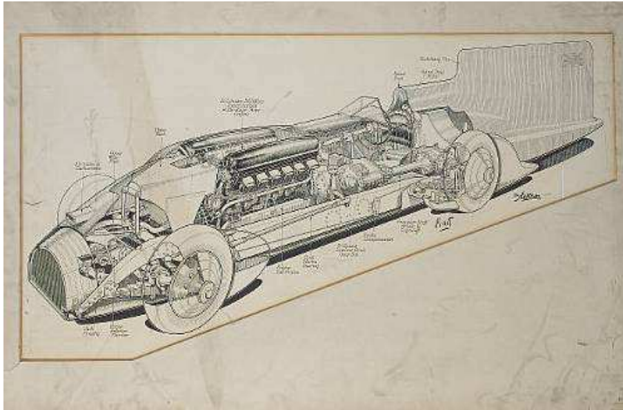
Bluebird cutaway 1933 Image courtesy of Bonhams
